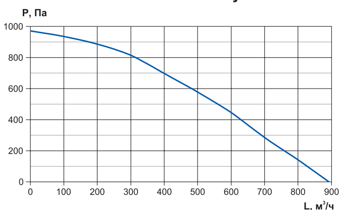
CV-SH-315-EC Grey
