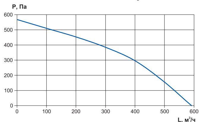
CV-SH-200-EC Grey
